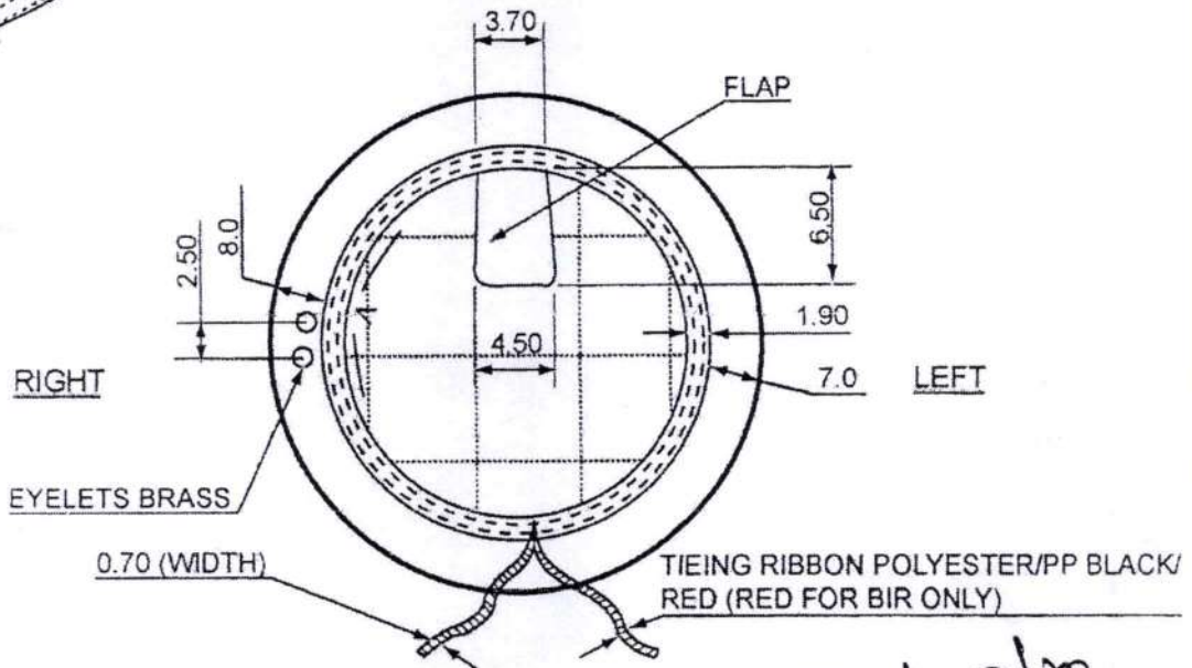
BACK VIEW
