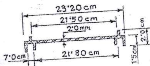
Plastic Lid (Section C-C)
