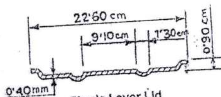
Single Layer Lid (Section B-B)
